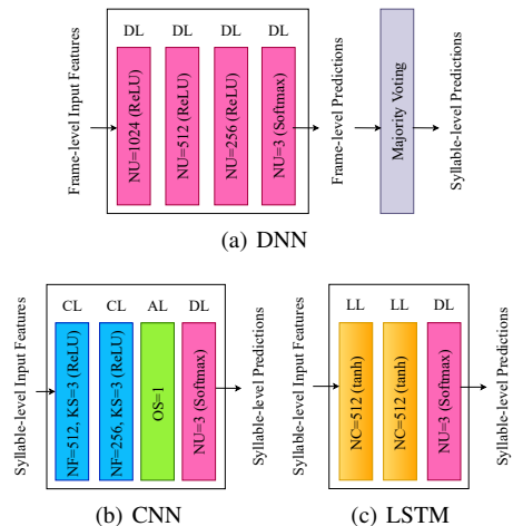
Figure 2: Architectures of different classifiers; here, DL: Dense layer, CL: 1D-Convolutional layer, AL: Adaptive average pooling layer, LL: LSTM layer, NU: Number of units in DL, NF: Number of filters, KS: Kernel size, OS: Output size of AL, NC: Number of LSTM cells
