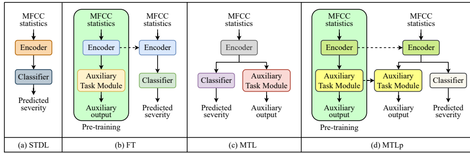
Figure 1: Block diagram of different network training protocols used in this work; here, dotted arrows indicate that the weights learned during pre-training are used as initializations in the next step
