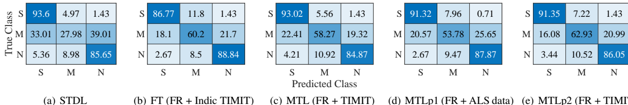
Figure 2: Confusion matrices averaged over 10-folds of random validation for STDL and the best performing configurations of the transfer learning approaches; here, S: Severe class, M: Mild class, N: Normal class; the entry in the cell (i, j) of each matrix indicates the % of samples of true class i which are being classified as class j
